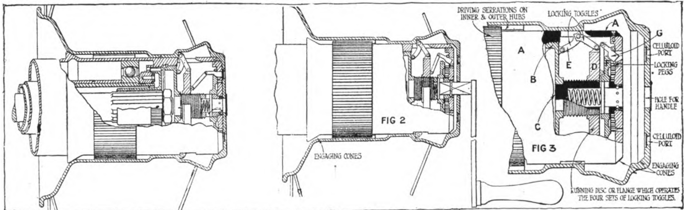
Fig. 1—Part sectional view of the Rapid detachable wheel. The locking mechanism is entirely enclosed within the outer end of the detachable hub. In this view the detachable hub is shown locked in position as in normal use. Fig. 2, showing the outer hub in the process of being forced "home" by the toggles, the operating handle being in position. Fig. 3 shows the locking mechanism in detail before the outer hub has been pushed on to the inner hub far enough for the toggles to be brought into action
